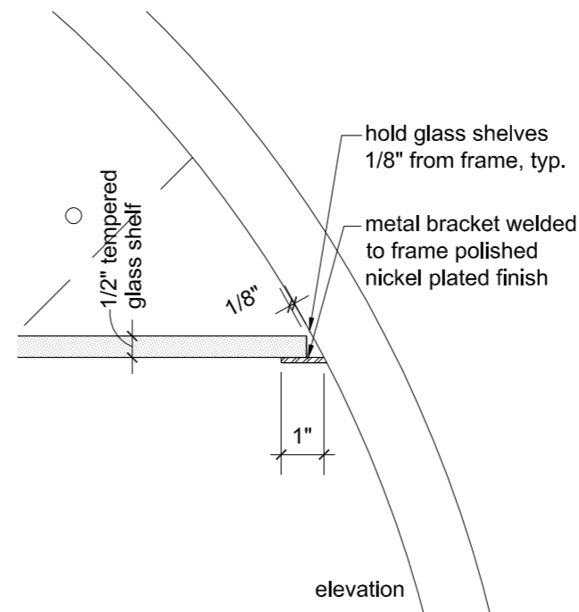
B detail at shelf brackets - elevation scale: 3" = 1'-0"
