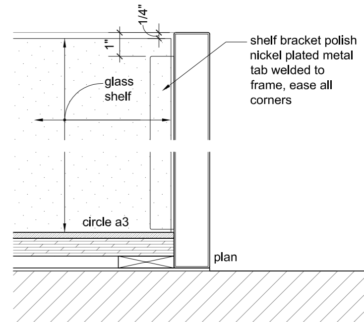
B detail at shelf brackets - plan scale: 3" = 1'-0"
